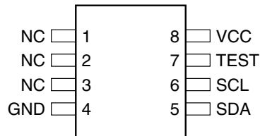
8-lead SOIC
